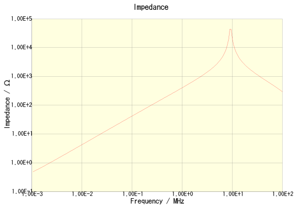
CLF10040T-680M-CA
