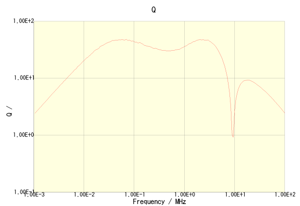
CLF10040T-680M-CA
