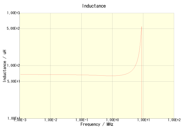
CLF10040T-680M-CA
